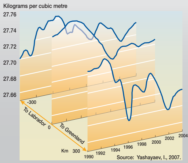
Depth corrected density of Labrador Sea water (northern North Atlantic) at 200-800 metre depth
