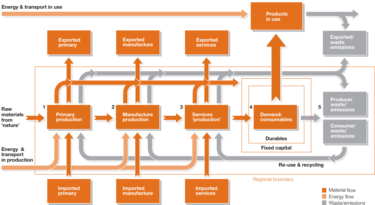
Fig 2 SCP framework
