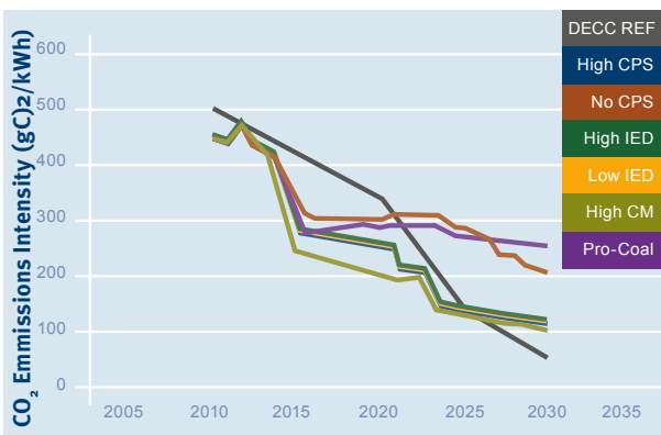
Figure 11: CO 2 emissions intentisty of grid electricity
